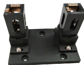
Single-hole cuvette holder (standard for double beam)
